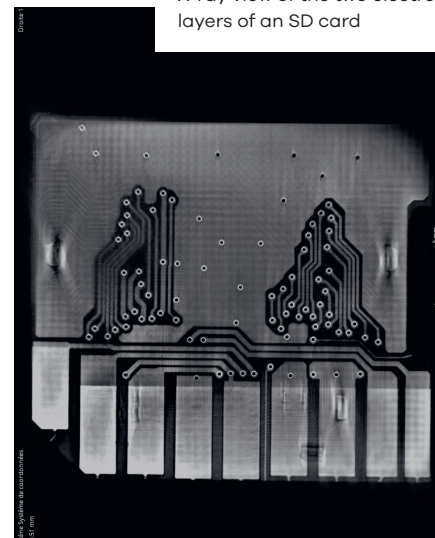
X-ray view of the two electronic layers of an SD card
